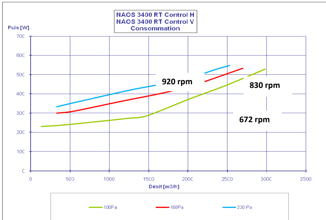
Figure 10 – NAOS 3400 RT CONTROL
