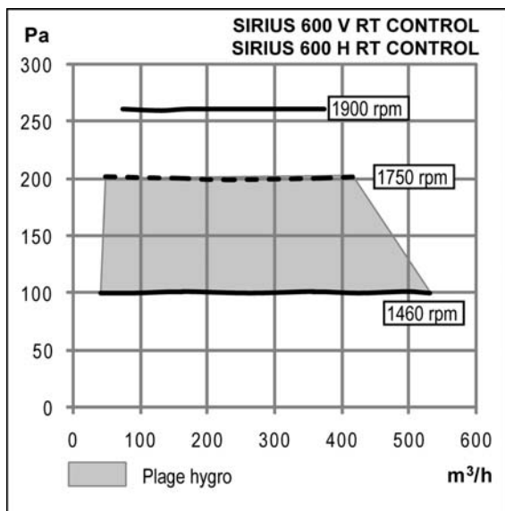
Figure 3 – SIRIUS 600 V RT CONTROL et SIRIUS 600 H RT CONTROL
