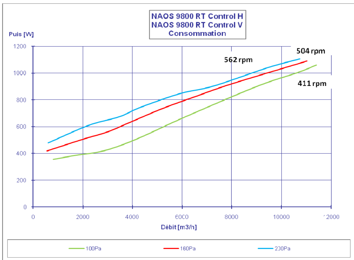
Figure 16 – NAOS 9800 RT CONTROL
