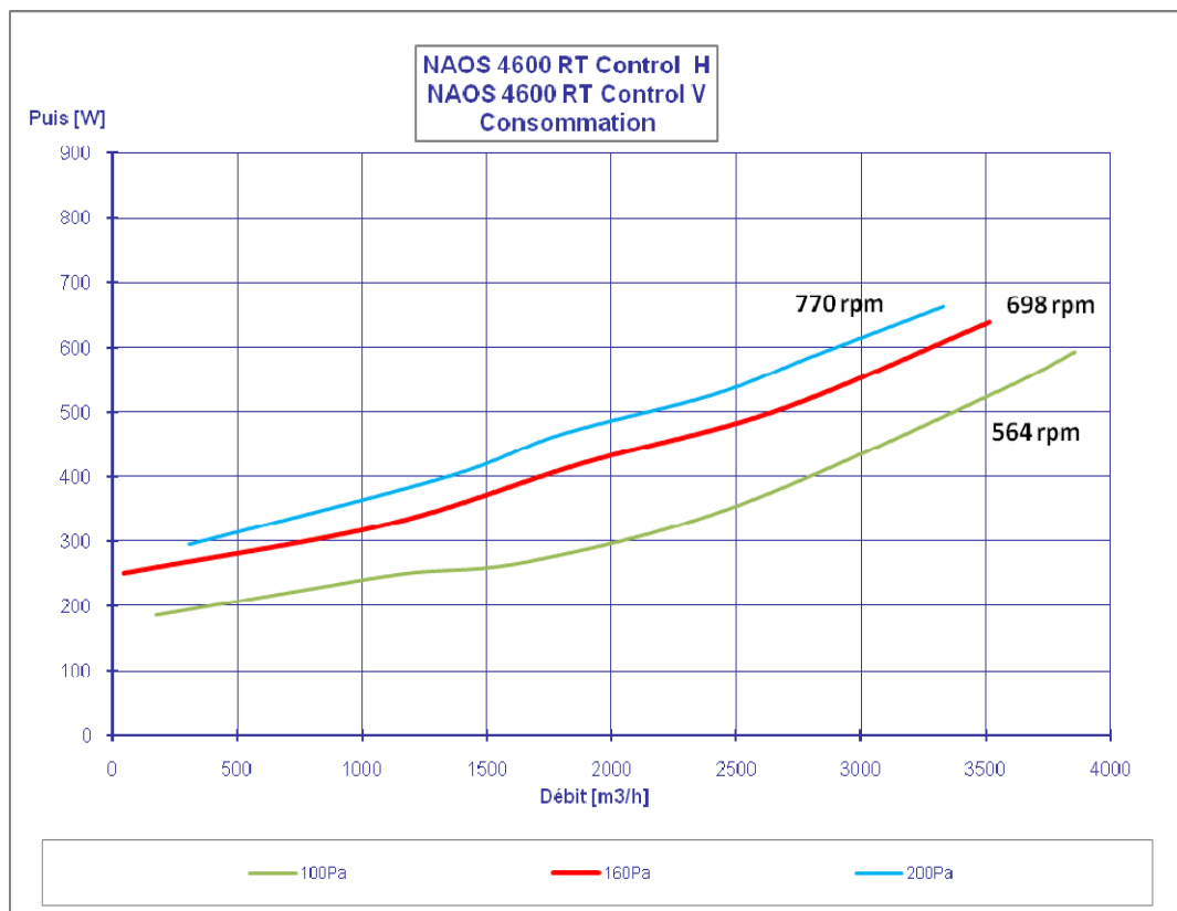
Figure 12 – NAOS 4600 RT CONTROL
