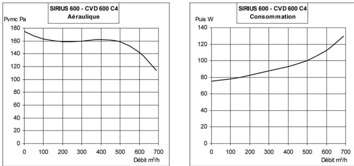
Figure 1 – SIRIUS 600 – CVD 600 C4
