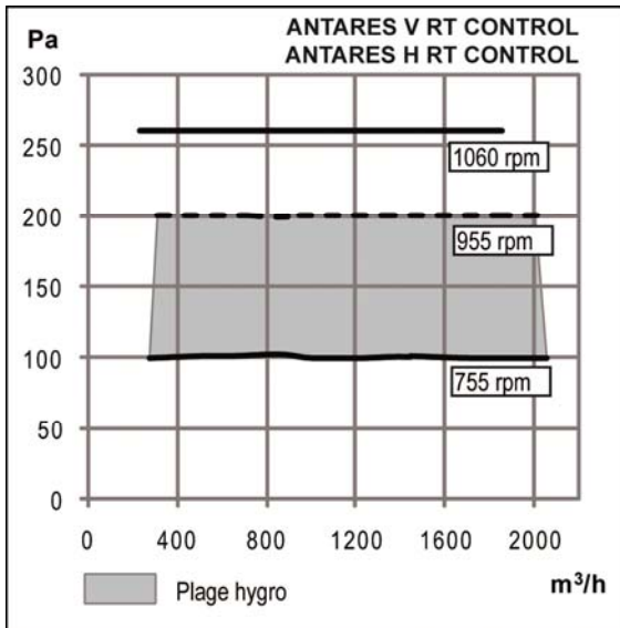
Figure 6 – ANTARES V RT CONTROL et ANTARES H RT CONTROL
