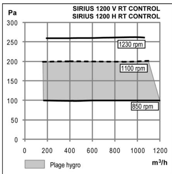
Figure 4 – SIRIUS 1200 V RT CONTROL et SIRIUS 1200 H RT CONTROL
