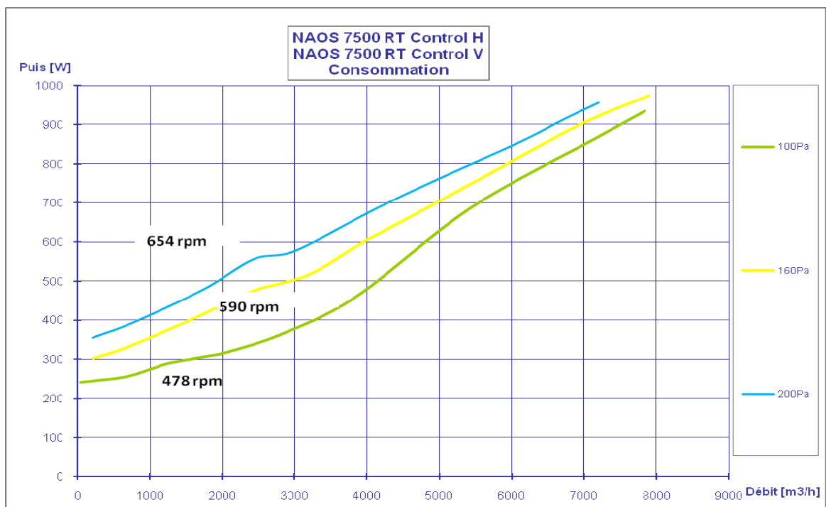
Figure 14 – NAOS 7500 RT CONTROL
