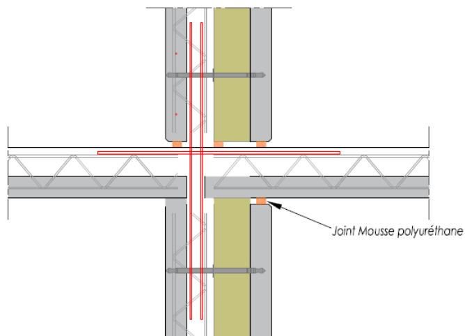
Figure 47 : Liaison Inov'Mur (i) /balcon
