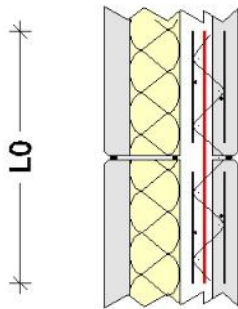
Figure 123 - 1 lit d'armatures verticales L0 = 2ls + 15 \text{ cm}
