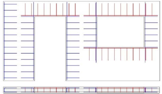
Figure 16 – Solution traditionnelle
