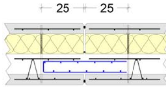
Figure 99 - 2 lits d'armatures
