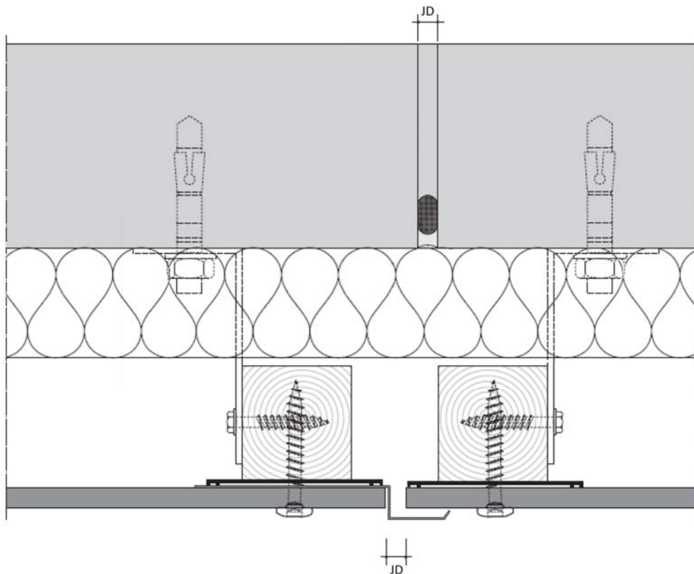
Figure 9 – Joint de dilatation
