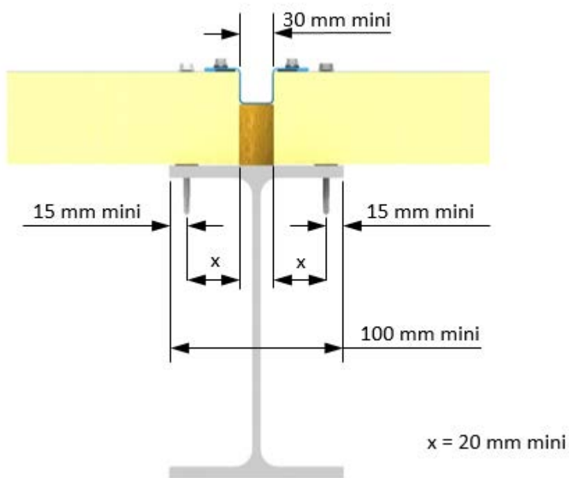
Figure 12 – Jonction verticale en pose horizontale – joint creux
