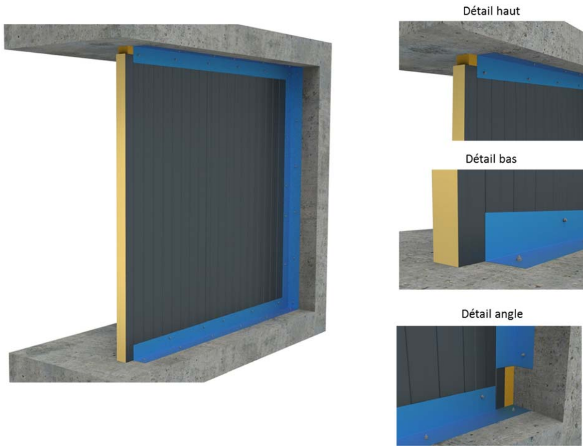
Figure 22 – Exemple de cloison – Pose verticale
