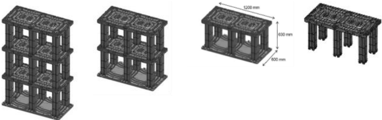
Figure 1a – Module WAVINQ-Bic Plus LC
