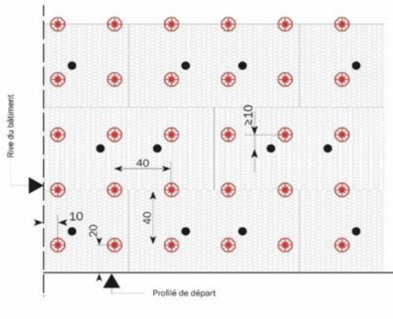
Figure 6a : Plan de chevillage 40 cm x 40 cm
