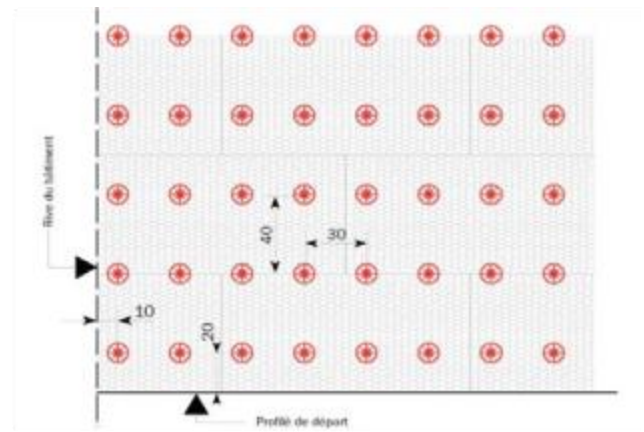
Figure 3b : Calepinage 40 cm x 30 cm
