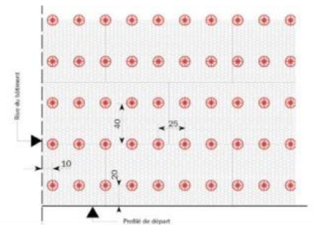
Figure 3c : Calepinage 40 cm x 25 cm
