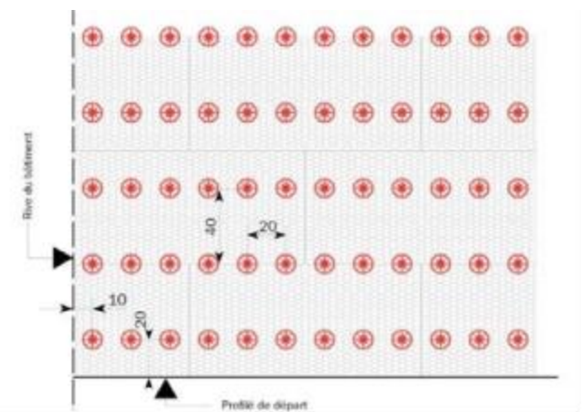
Figure 3d : Calepinage 40 cm x 20 cm
