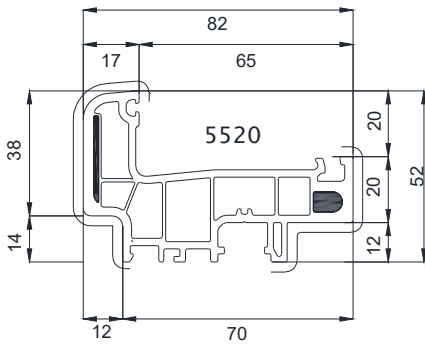
5520 I_x: 2.41\text{cm}^4 I_y: 0.27\text{cm}^4 inertie totale equivalent acier
