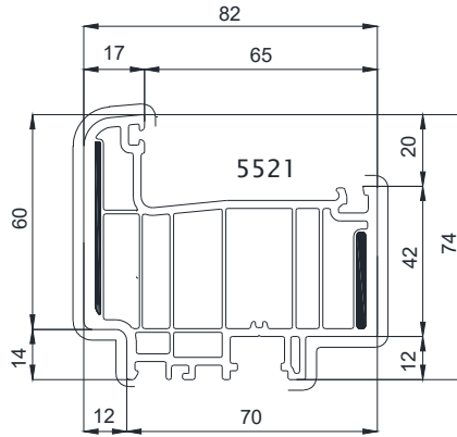
5521 I_x: 4.06\text{cm}^4 I_y: 0.97\text{cm}^4 inertie totale equivalent acier
