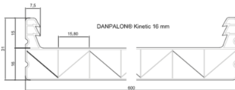
Figure 1.2 – Panneaux DANPALON® 35 mm et panneaux DANPALON® 3Dlite 16mm, 3Dlite 22mm et Kinetic 16mm
