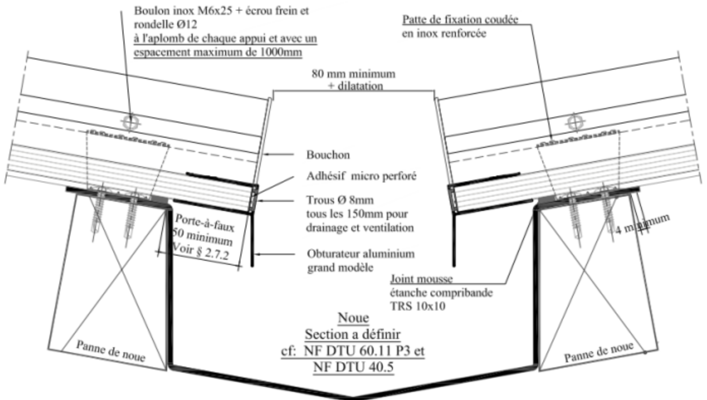
Figure 11 - Point particulier – Noue
