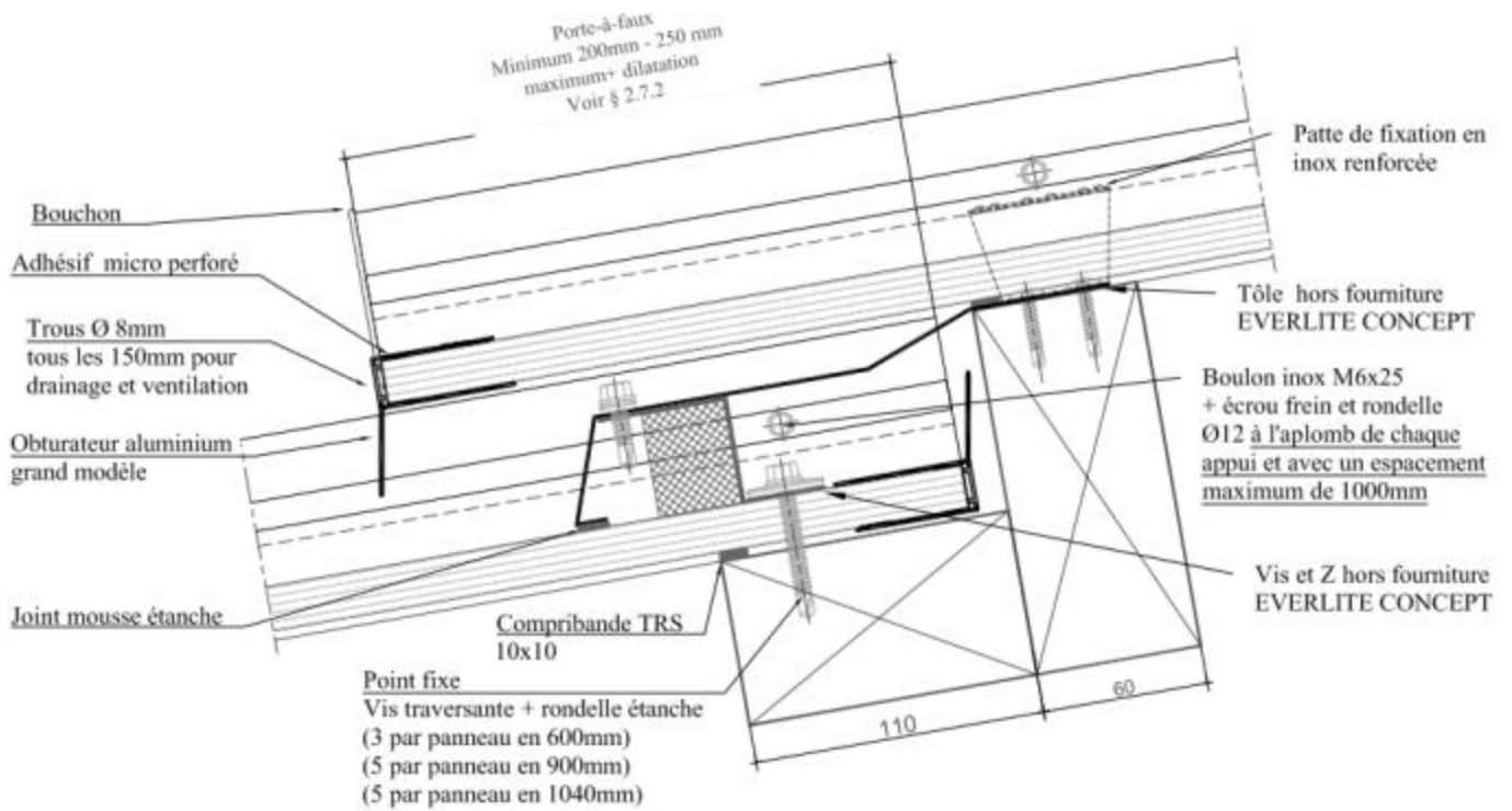
Figure 12 - Point particulier – Ressaut cf. § 2.7.4.5
