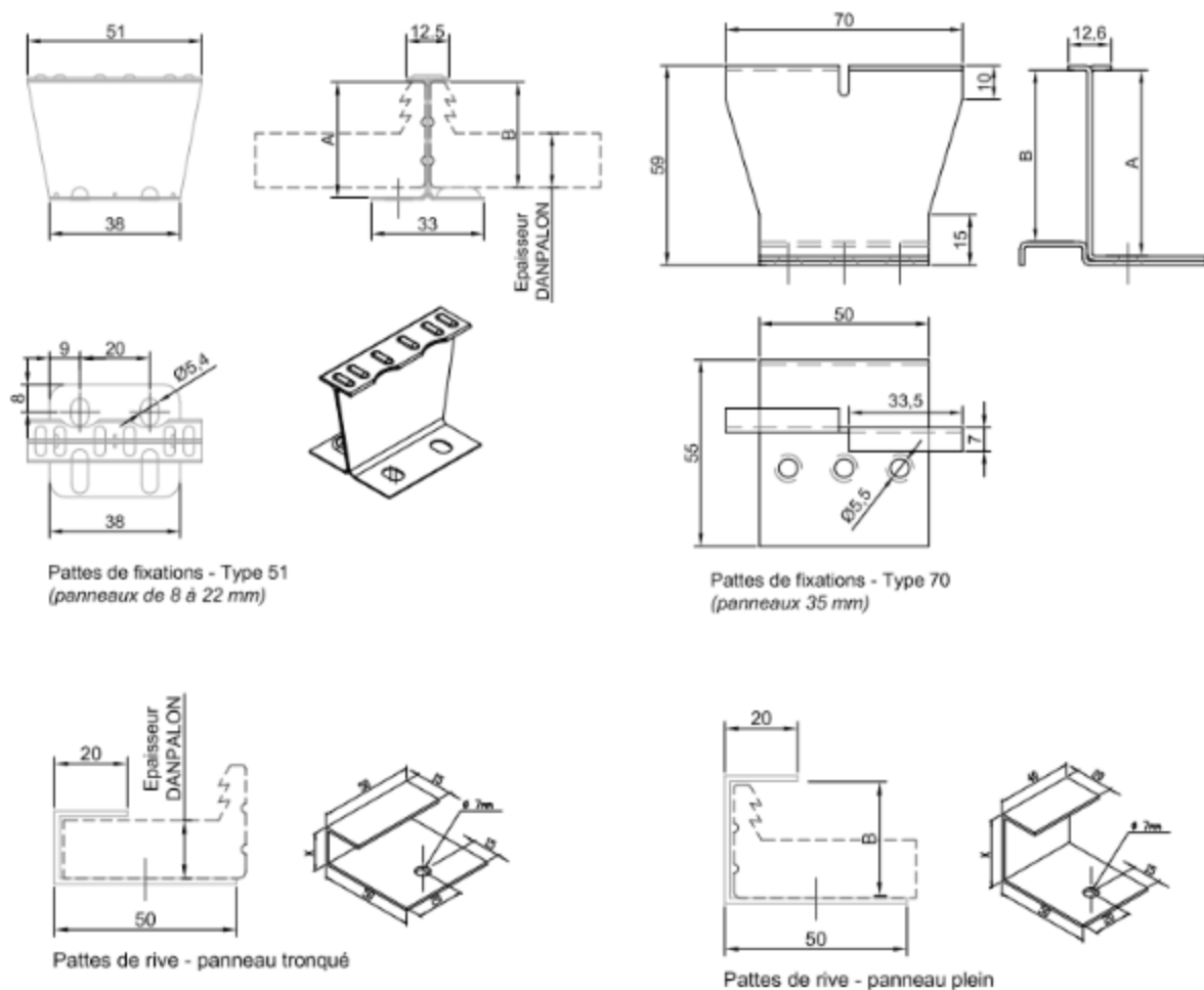
Figure 4.1 – Pattes de fixation
