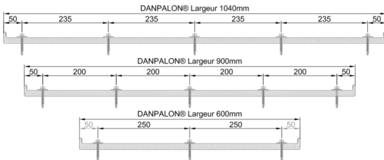
Figure 8 - Point particulier – Point fixe (point haut)
