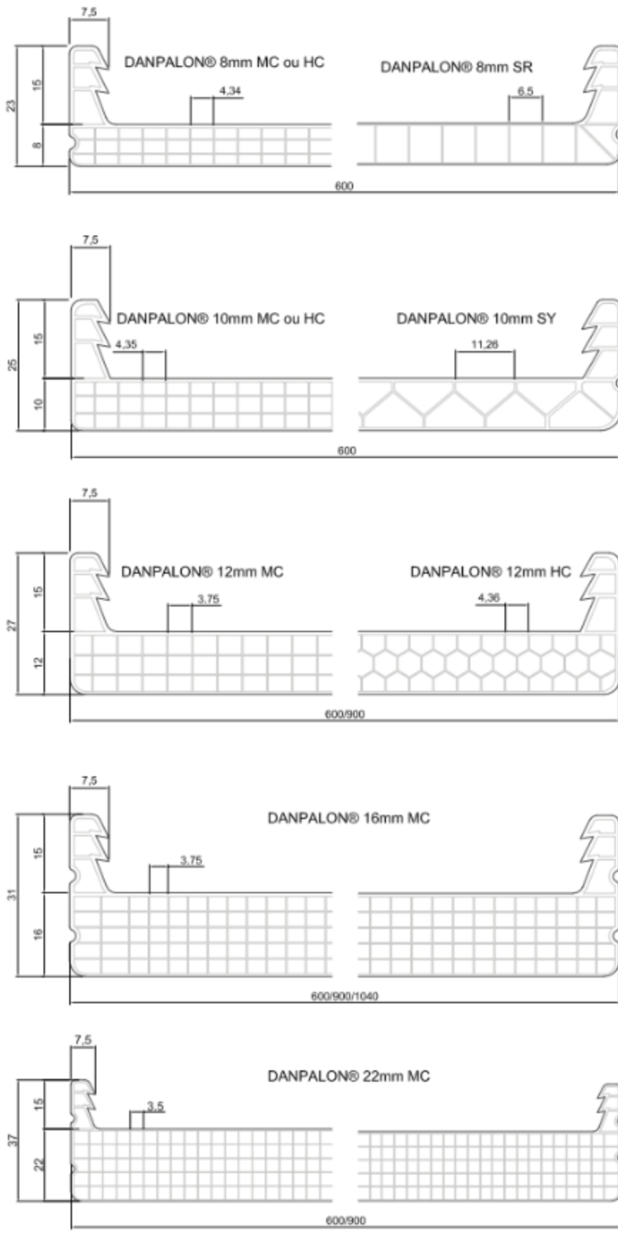
Figure 1.1 – Panneaux DANPALON® 8 mm, 10 mm, 12 mm, 16 mm et 22 mm
