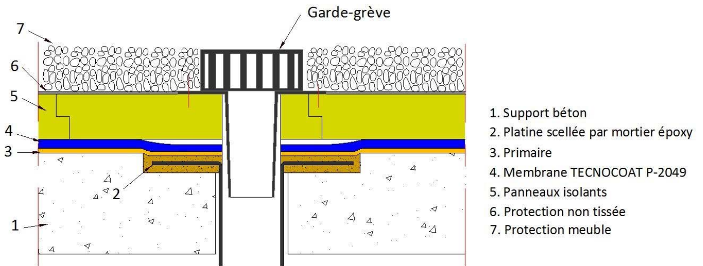
Figure 15 – Isolation inversée
