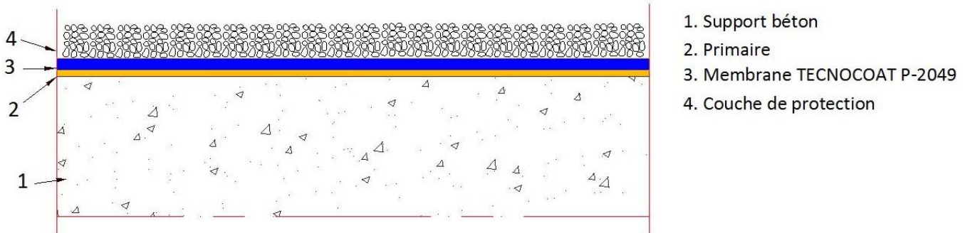
Figure 14 – Protection lourde meuble (granulats)
