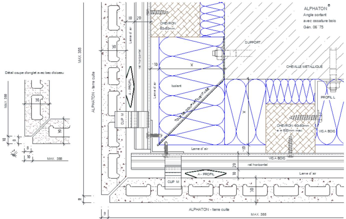
Figure 35 - Angle sortant
