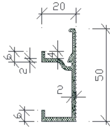
Figure 6 - Rail portant horizontal 06'75
