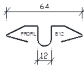
Figure 4 - Profilés de joint ressort vertical
