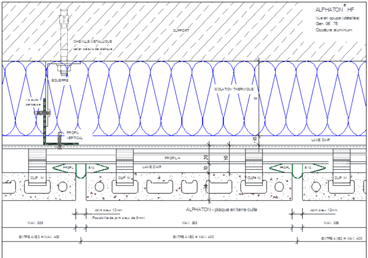
Figure 11 - Coupe horizontale
