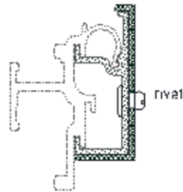
Figure 6 - Rail portant horizontal 06'75
