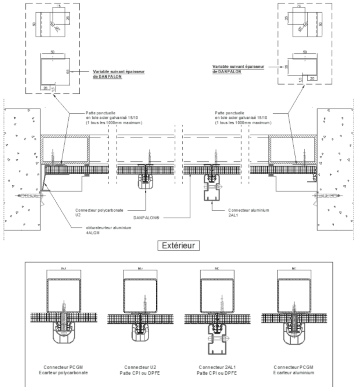
Figure 9 - Coupe horizontale
