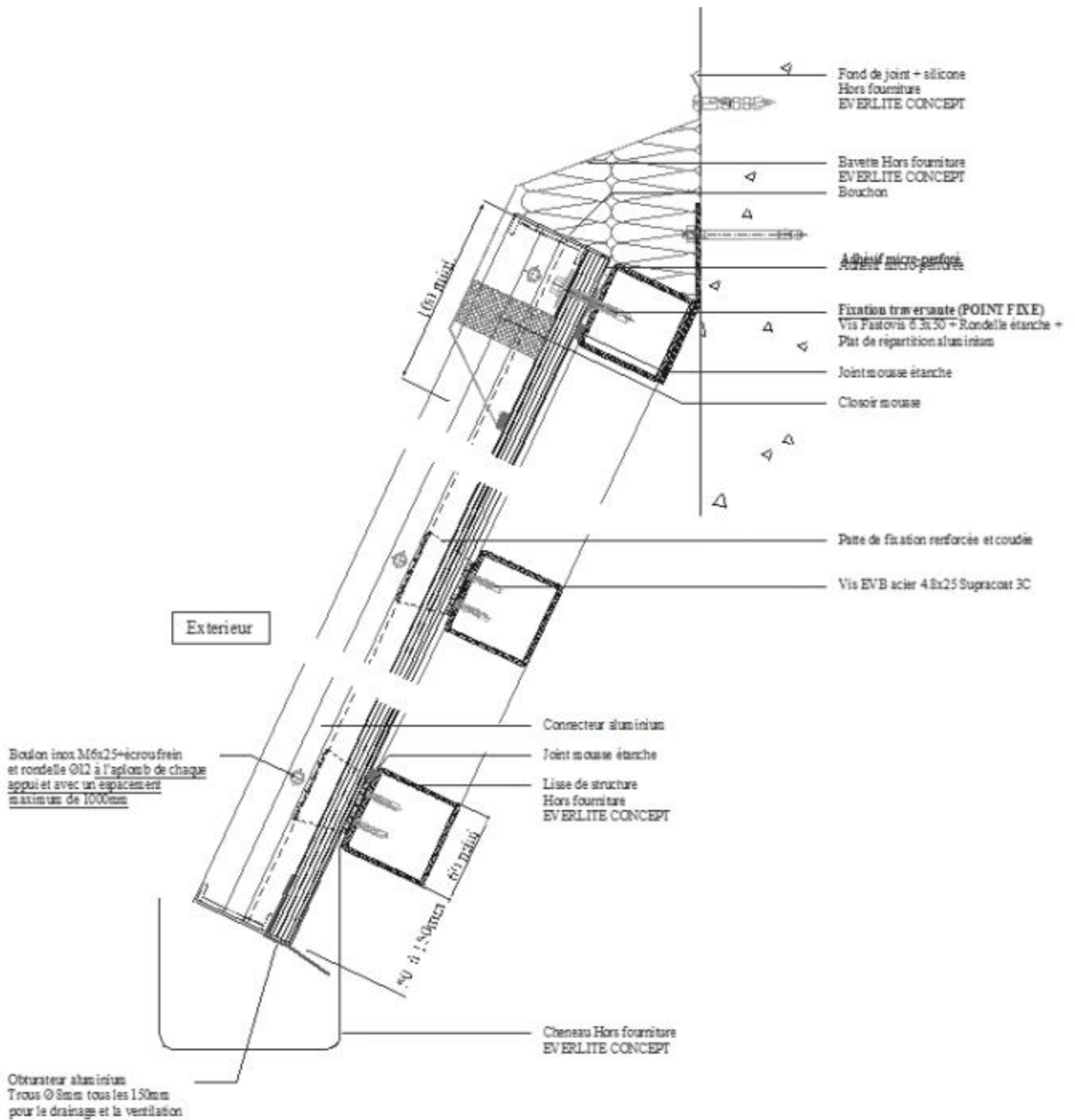
Figure 8.2 - Coupe verticale inclinée (SHED)
