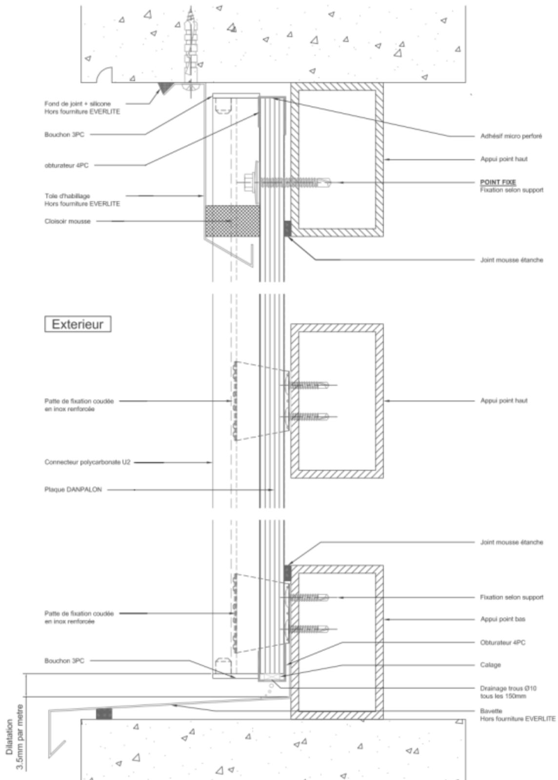
D Figure 8.1 - Coupe verticale
