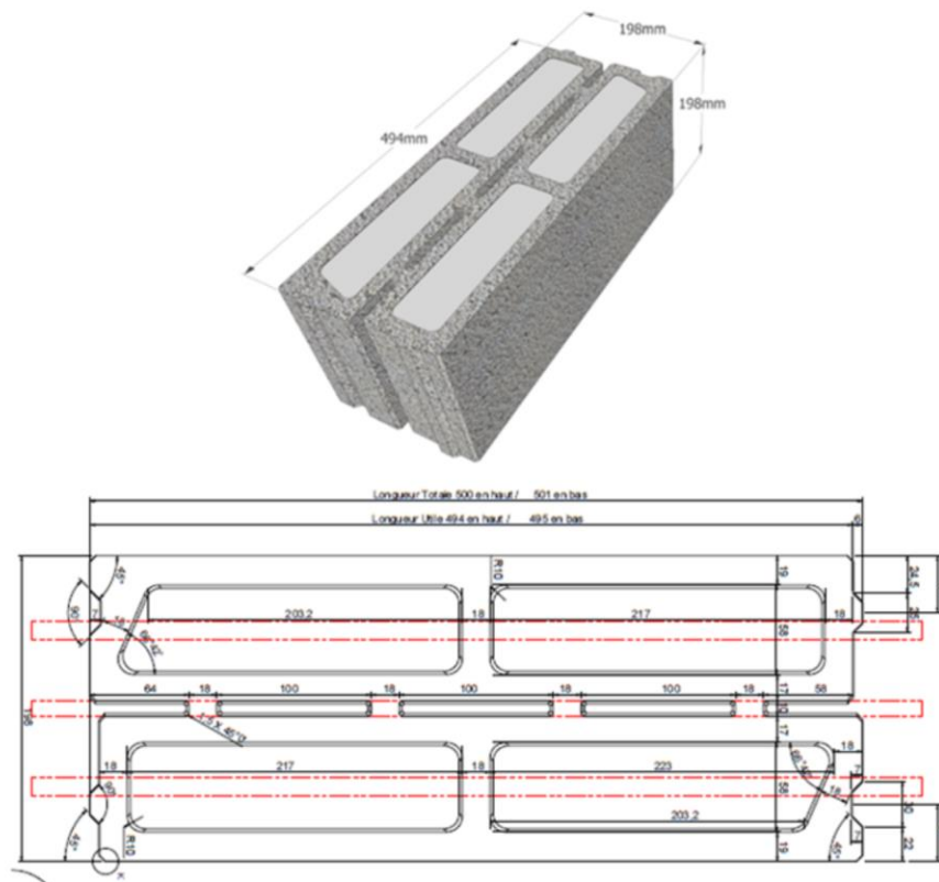
Figure 1 – FABTHERM AIR 1.1
