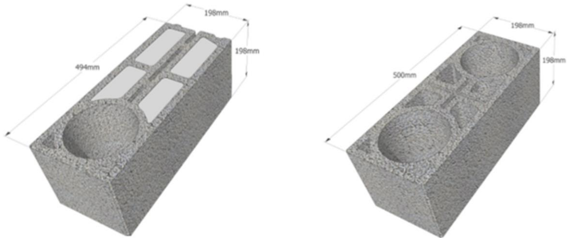
Figure 3 – FABTHERM AIR 1.1 angle et double angle
