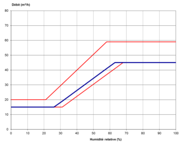
Figure 21 – C8 (15-45 m 3 /h, 26-63%HR)
