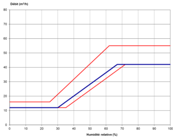
Figure 20 – C7 (12-42 m 3 /h, 30-67%HR)
