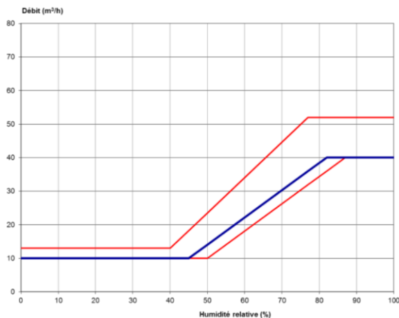
Figure 18 – C5 (10-40 m³/h, 45-82%HR)
