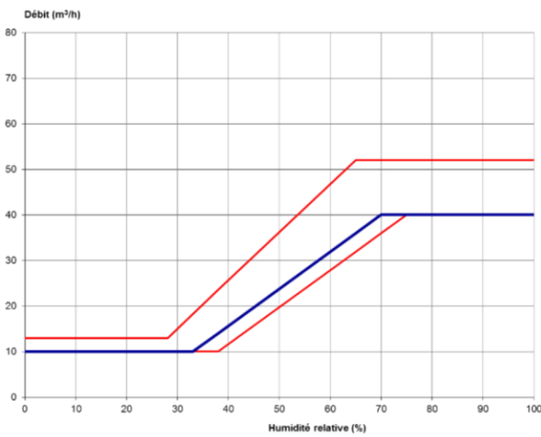
Figure 22 – B5 (10-40 m 3 /h, 33-70%HR)
