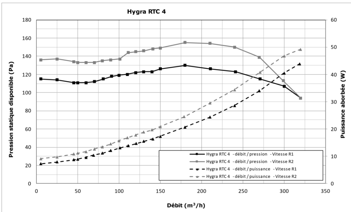
Figure 2 – Hygra RTC 4
