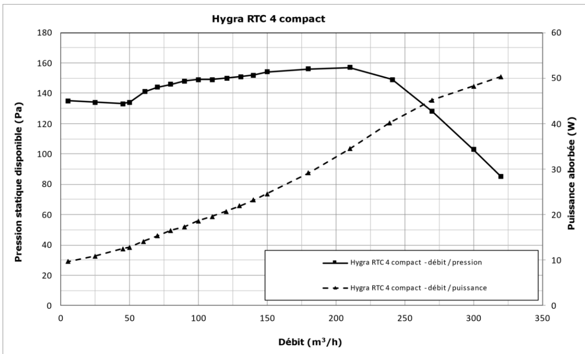
Figure 1 – Hygra RTC 4 compact
