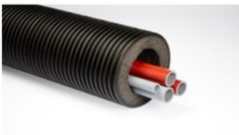
Figure 2 - Flexalen Multiline
