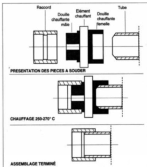
Figure 7 - Principe de soudage
