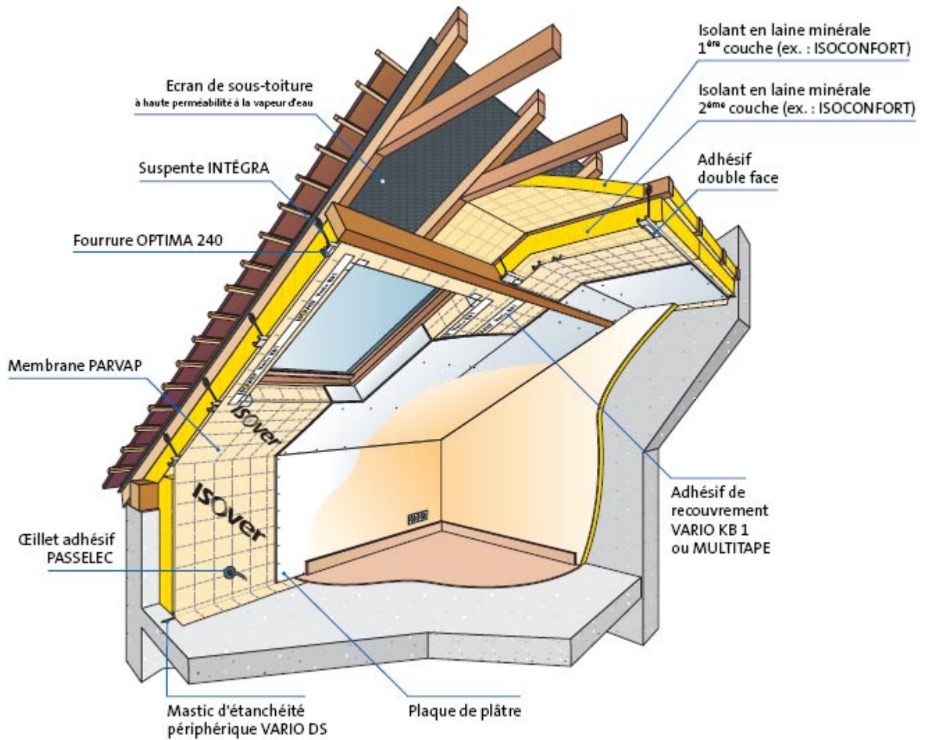
Figure 52 – Pose du parement
