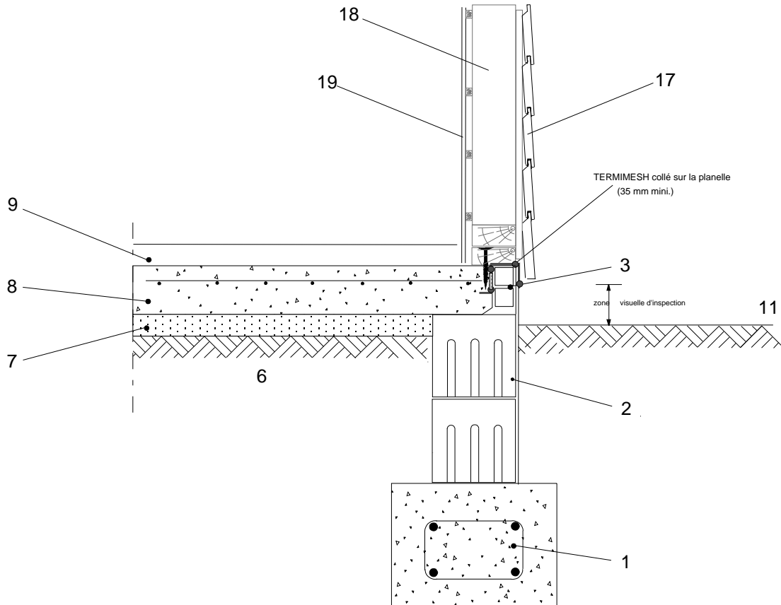
Figure 4 – EU 1.1-4_ dallage-ossature-bois_option1
