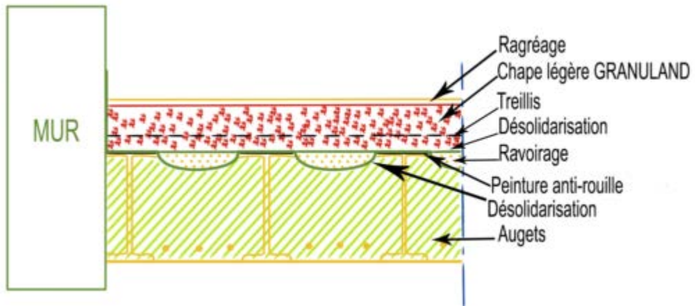
Figure 4 – Support plancher à augets
