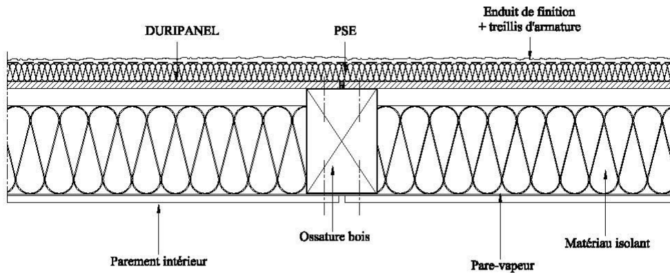
Figure 9 - Coupe sur joint vertical
